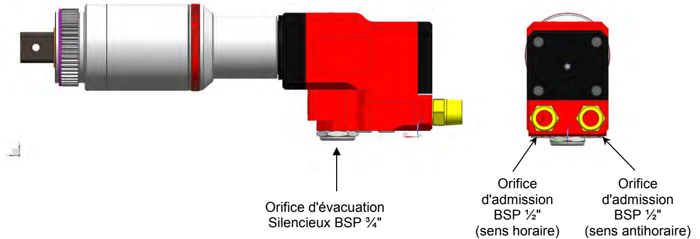
FIGURE 9 – Orifices
