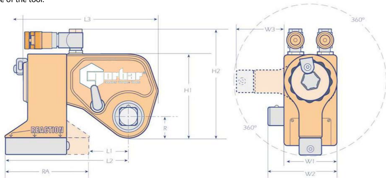
Square Drive - Tool Specifications
