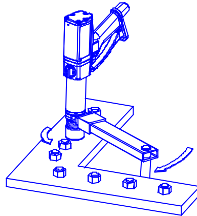
Figure 2b (Counter-clockwise)
