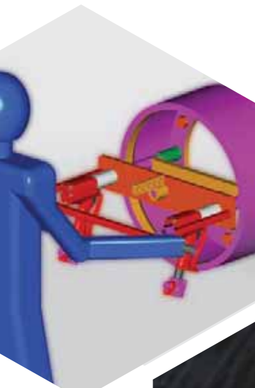
Twin spindle unit comprising of a Pneutorque® stall tool, special nose extensions, reaction plates and frame
